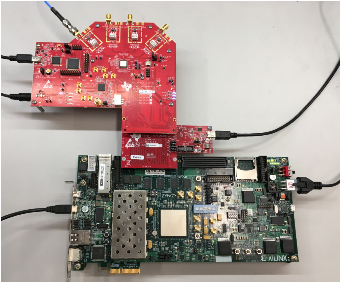
Figure 26. DAC38J84EVM, TSW14J10EVM and ZC706 Board
