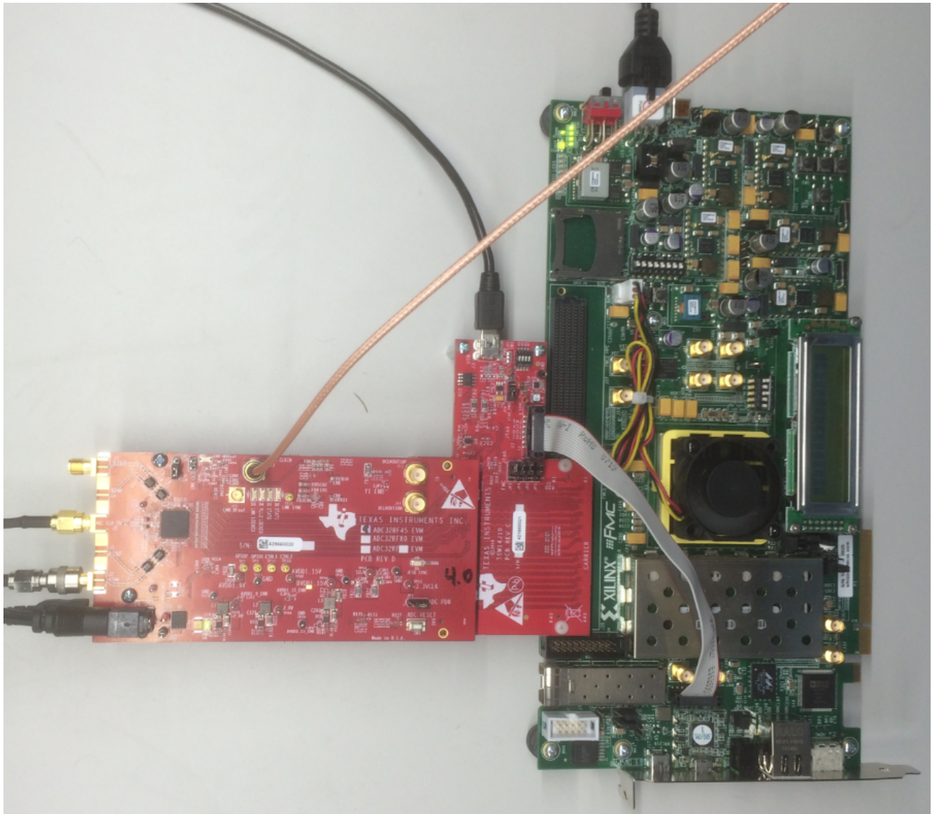
Figure 13. ADC32RF45EVM, TSW14J10EVM and VC707 Board
