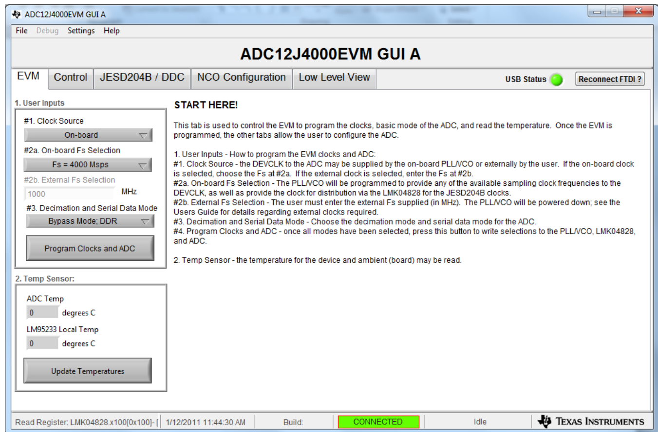
Figure 19. ADC12J4000EVM GUI
