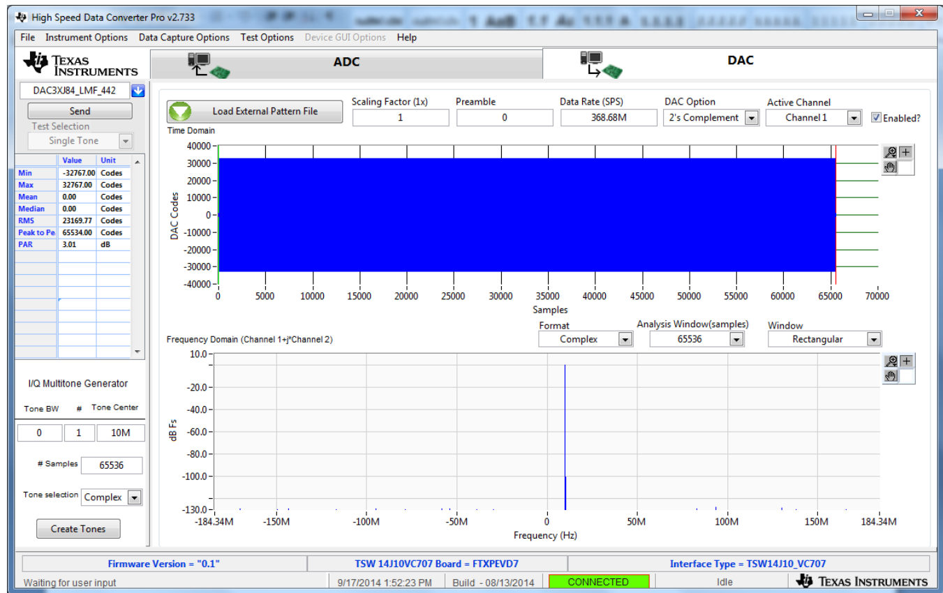
Figure 28. HSDC Pro GUI
