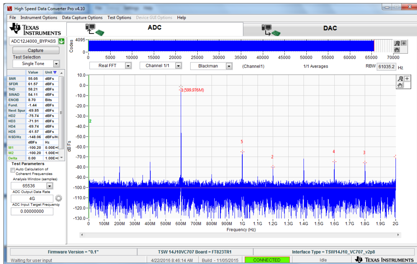
Figure 25. Captured Results for the ADC12J4000 in Bypass Mode
