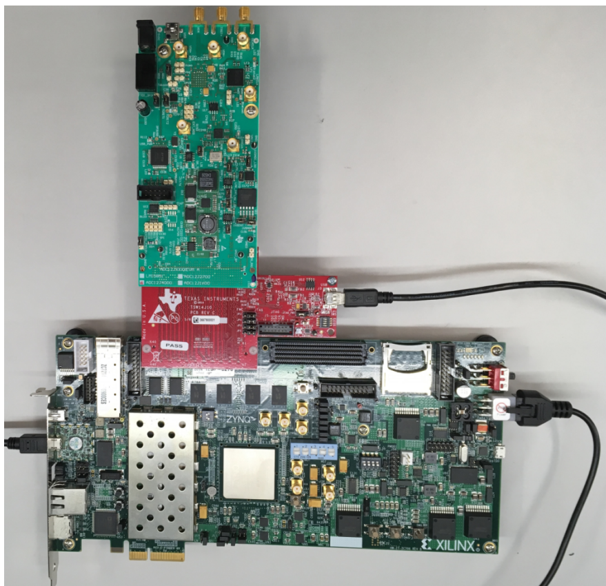
Figure 24. ADC12J4000EVM, TSW14J10EVM and ZC706 board
