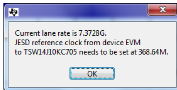
Figure 29. HSDC Pro GUI
