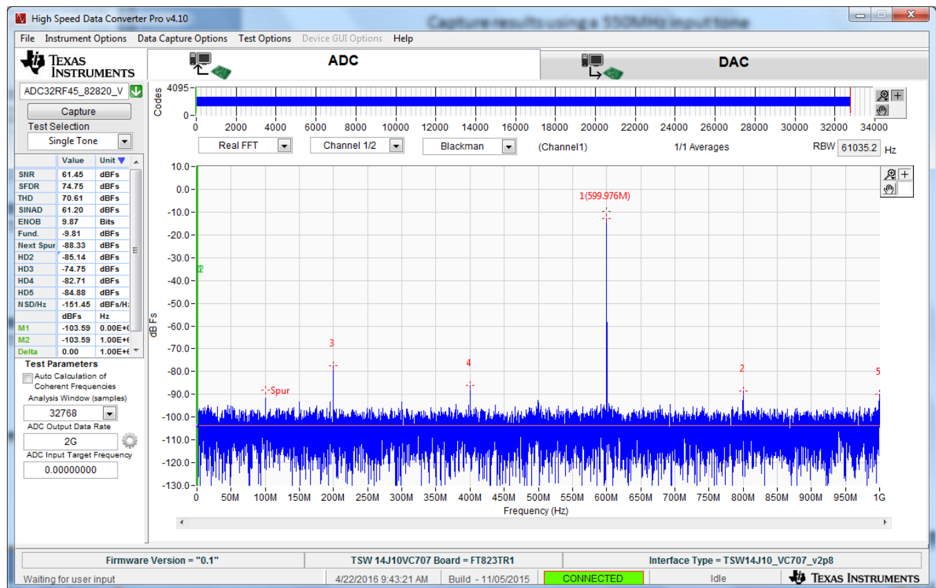
Figure 17. Captured Results for Channel A
