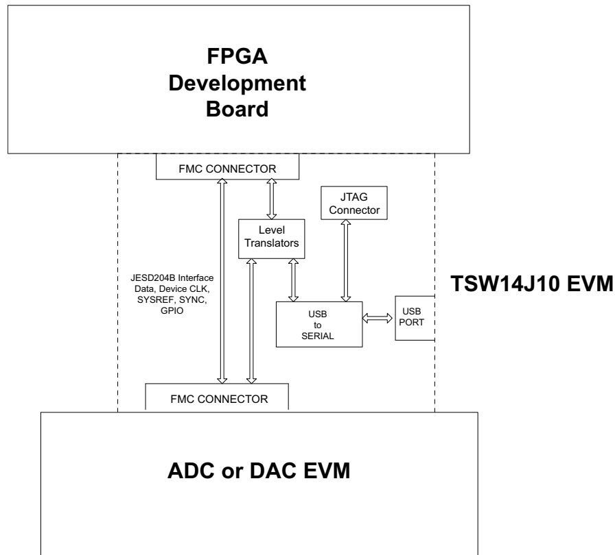
Figure 2. TSW14J10 EVM Block Diagram
