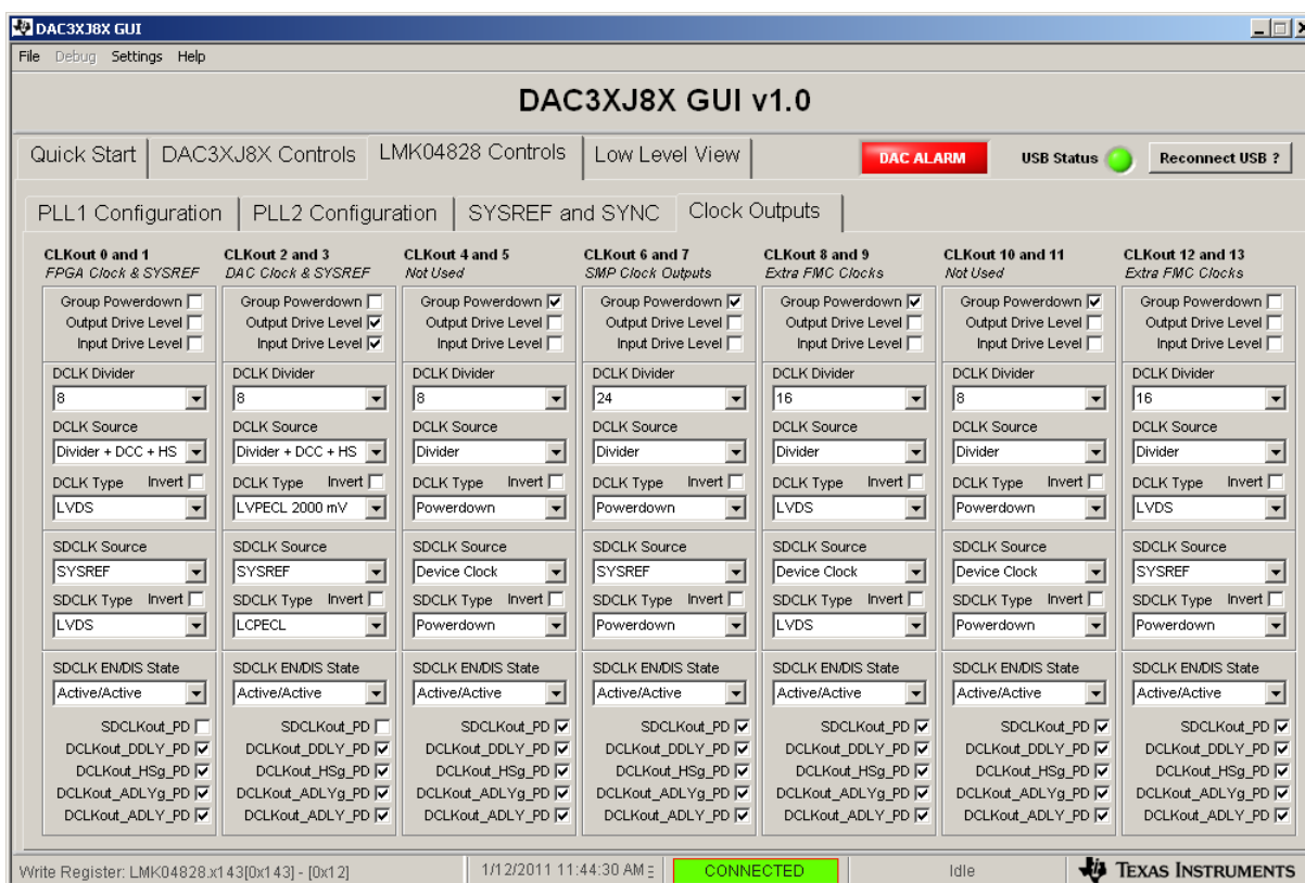
Figure 10. LMK04828 Clock Outputs Menu
