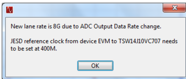
Figure 16. HSDC Pro GUI
