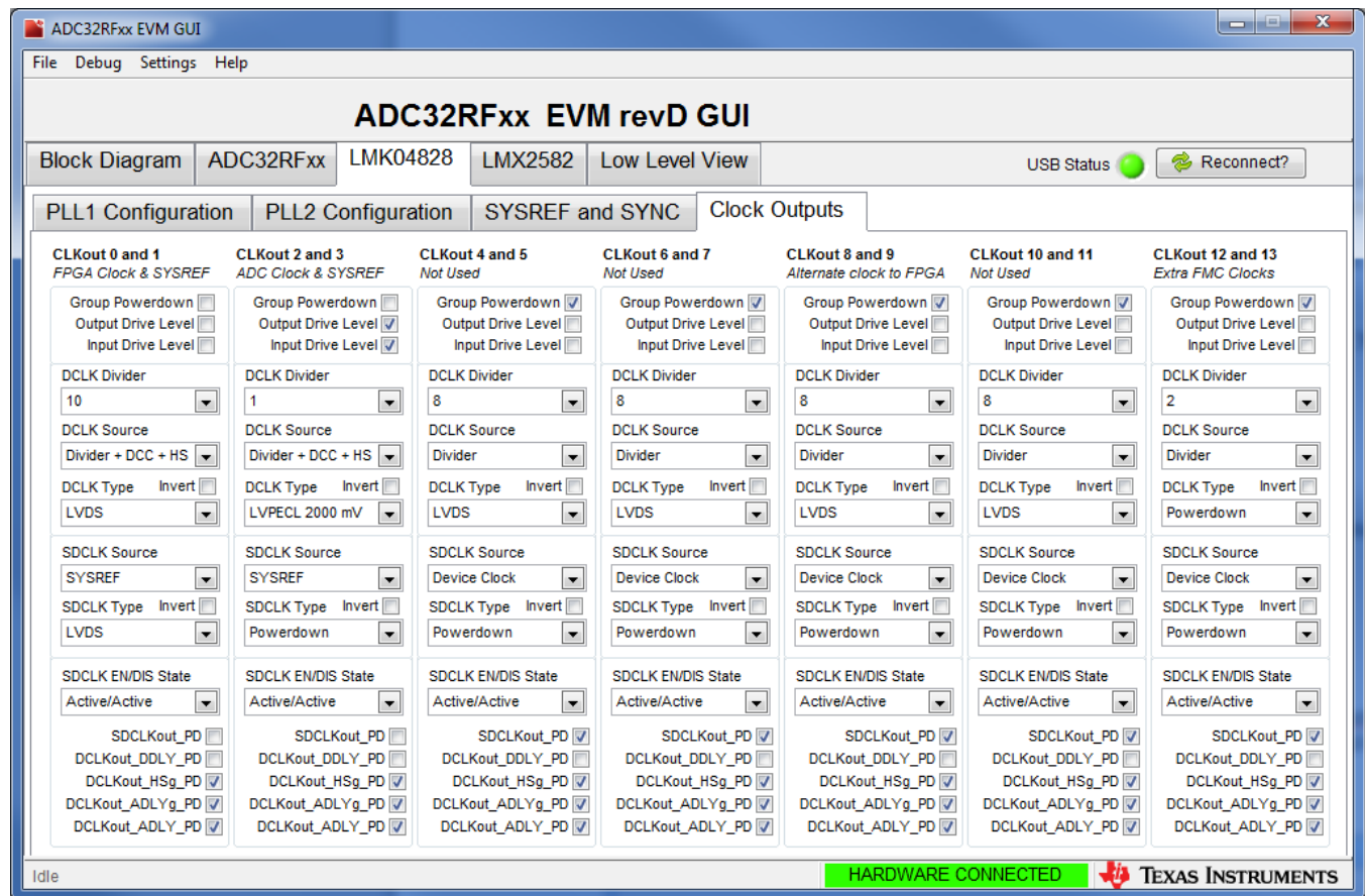
Figure 14. ADC32RFxx GUI LMK0828 Clock Outputs Tab
