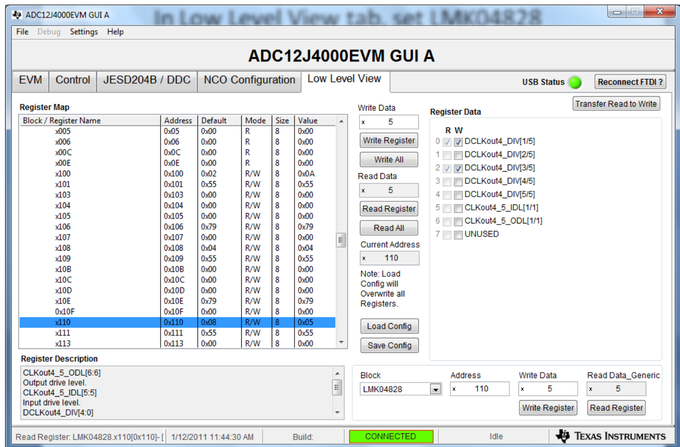
Figure 21. LMK04828 Address 0x110
