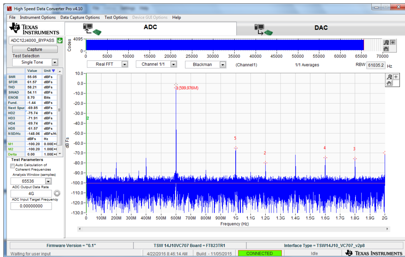
Figure 23. Captured Results for the ADC12J4000 in Bypass Mode
